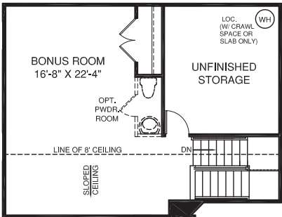
OPT. SECOND FLOOR W/ OPT. BONUS ROOM
