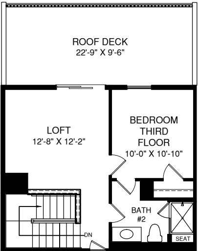
OPT. BEDROOM THIRD FLOOR W/ OPT. 4' EXT. TO HOUSE
