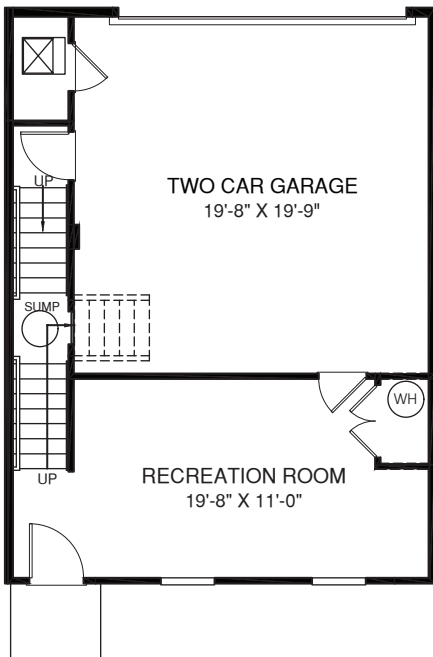
LOWER LEVEL
