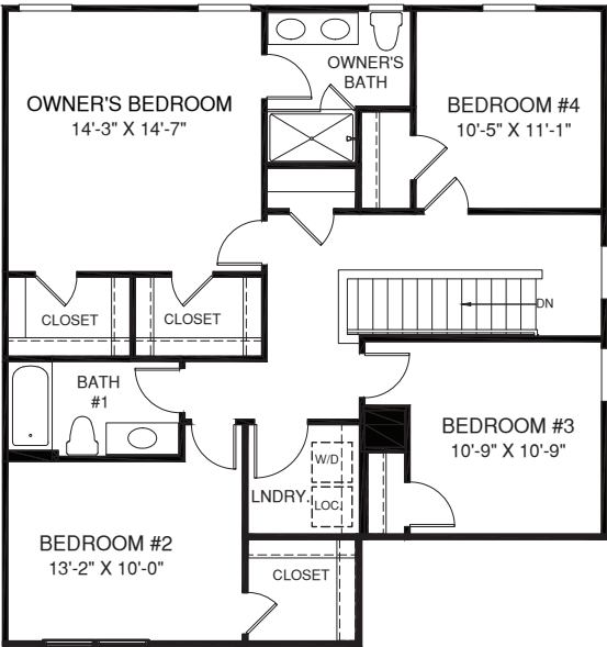
UPPER LEVEL
