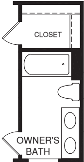
OPT. OWNER'S BATH W/ DOUBLE BOWL VANITY
