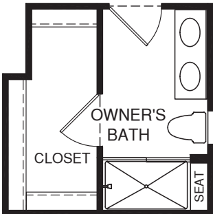
OPT. OWNER'S BATH ALTERNATE LAYOUT
