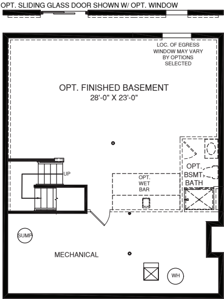
LOWER LEVEL
