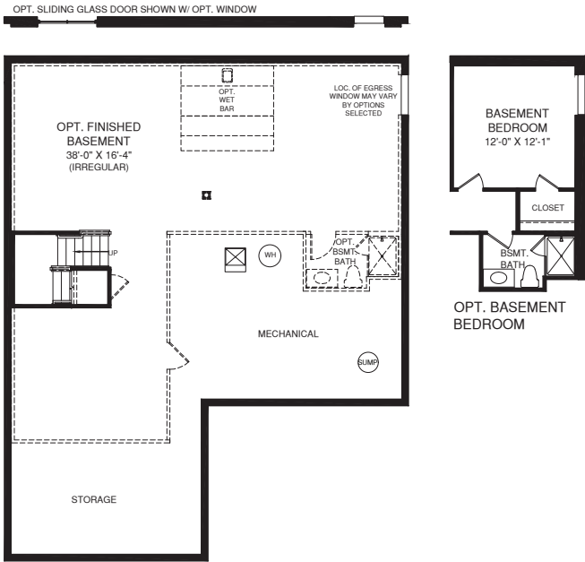
LOWER LEVEL
