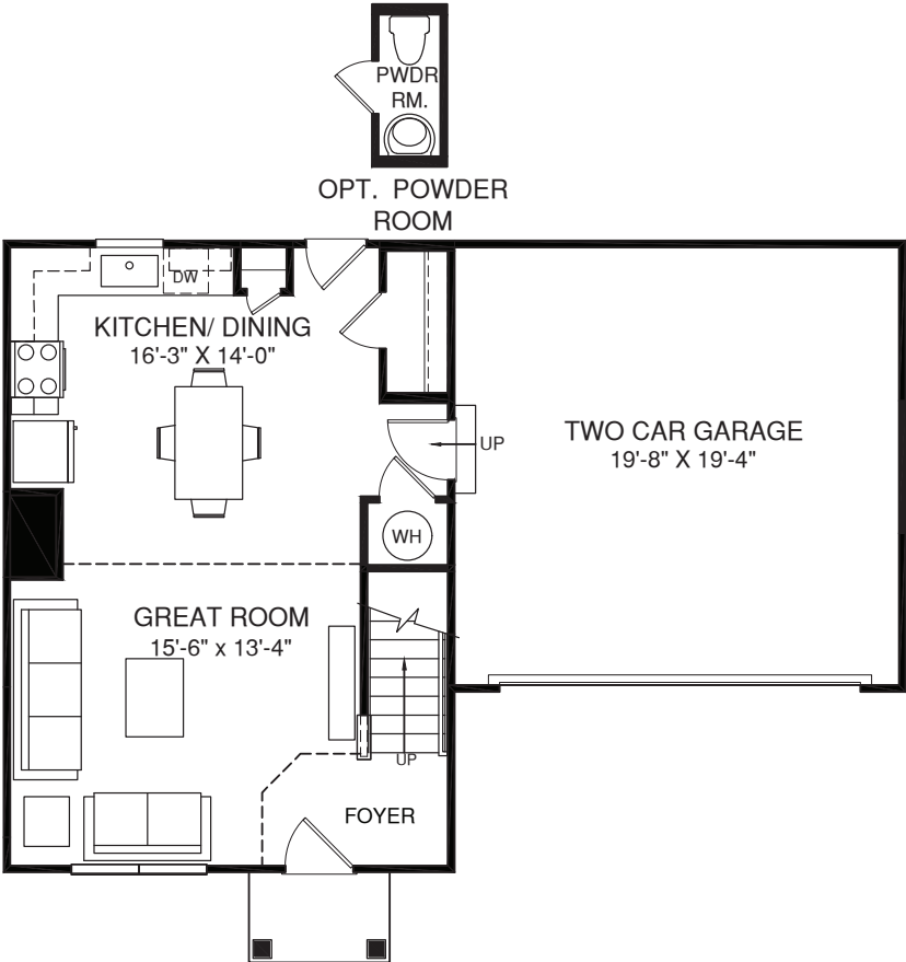
MAIN LEVEL
