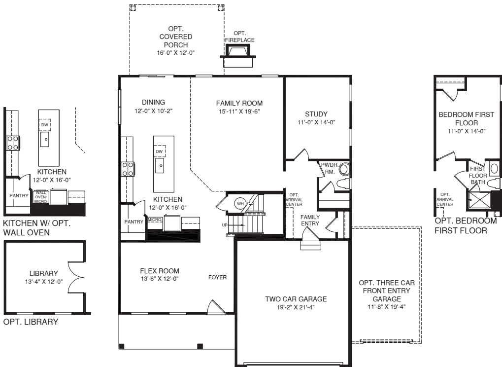
MAIN LEVEL
