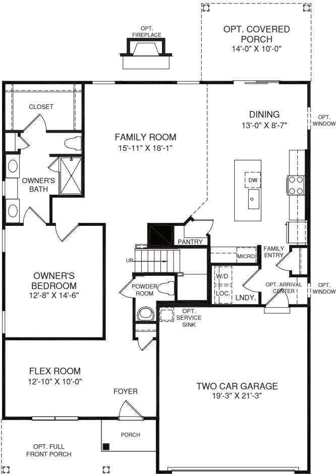
MAIN LEVEL
