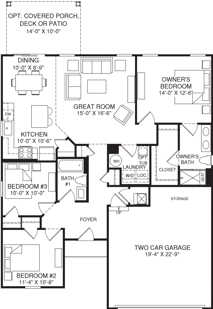
MAIN LEVEL
