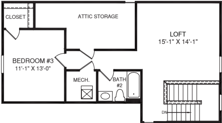
OPT. UPPER LEVEL
