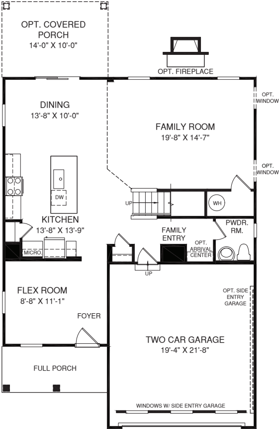
MAIN LEVEL
