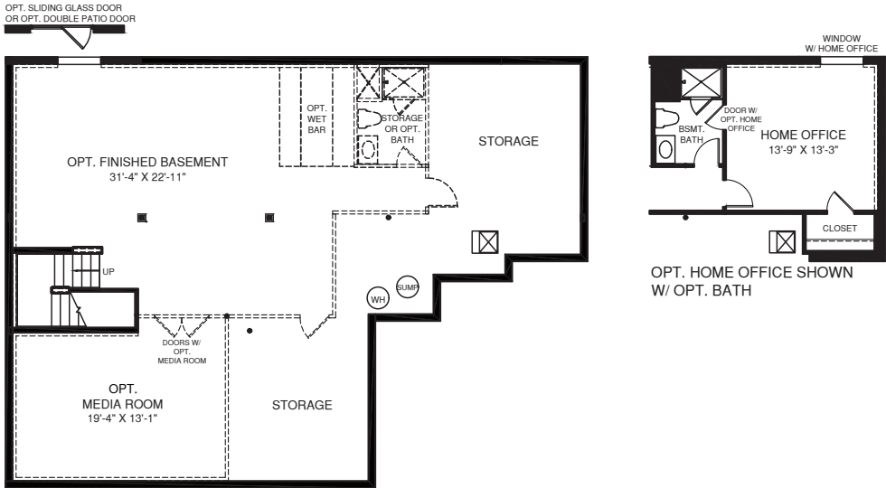
LOWER LEVEL
