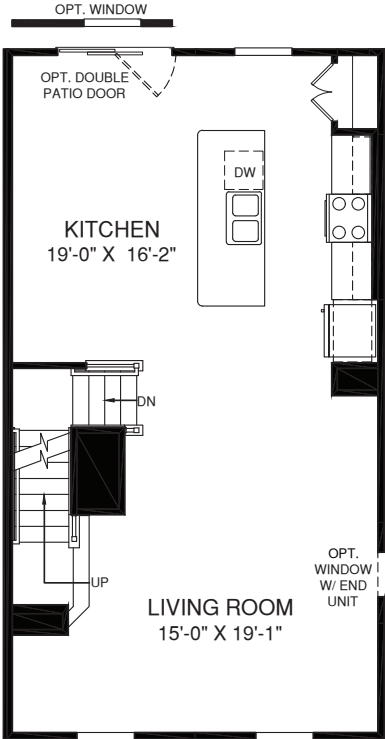
MAIN LEVEL
