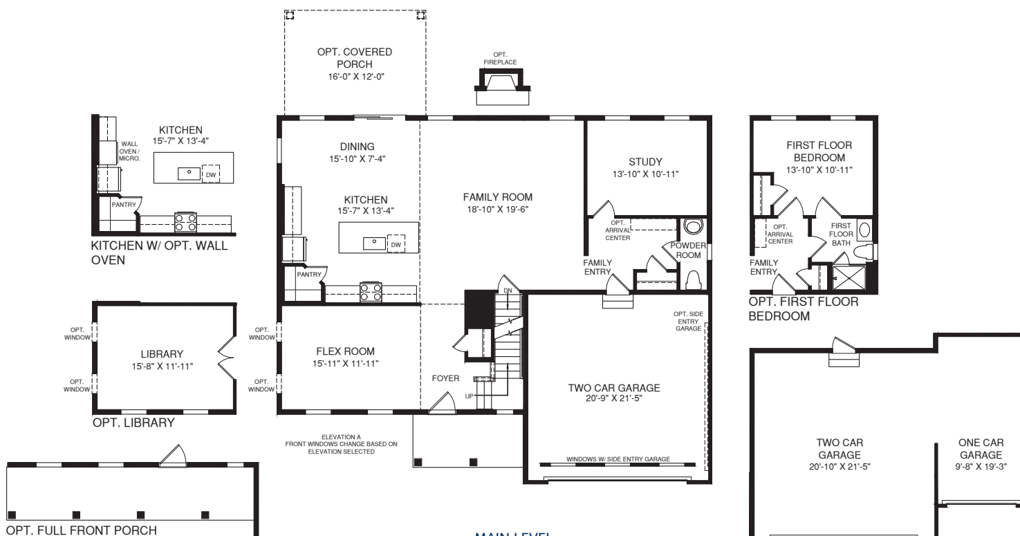
OPT. THREE CAR GARAGE
