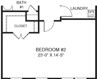
OPT. 2 BEDROOM LAYOUT
