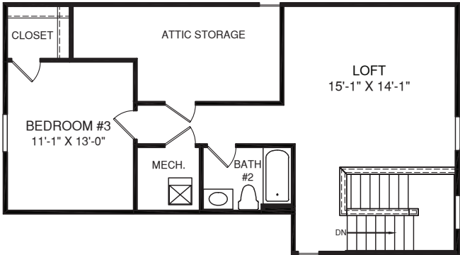
UPPER LEVEL
