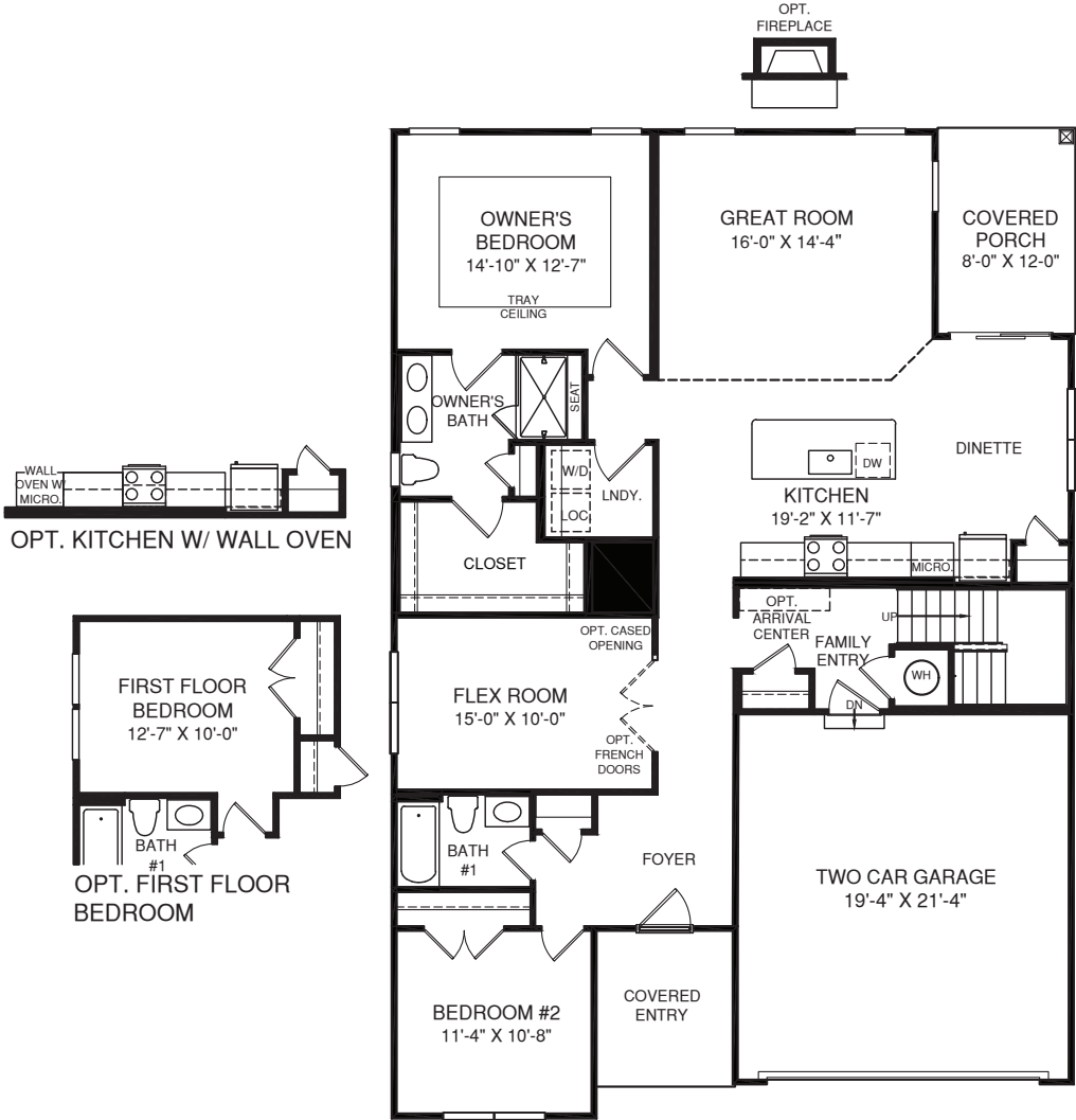
MAIN LEVEL
