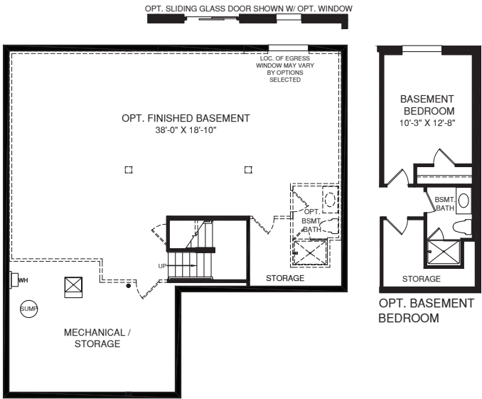
LOWER LEVEL
