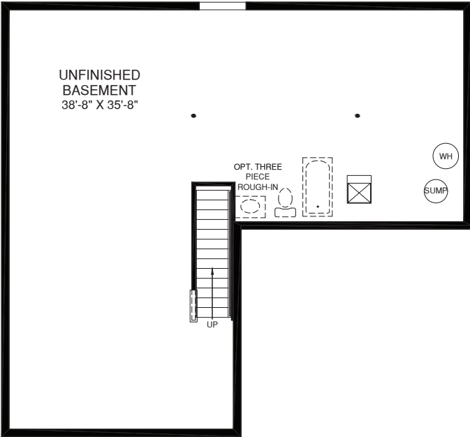
LOWER LEVEL
