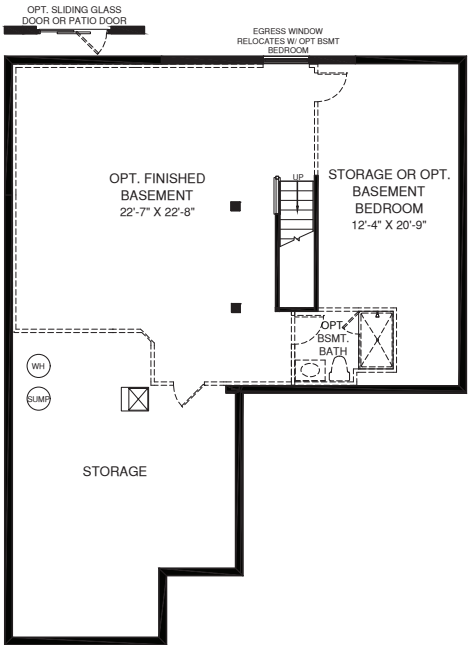
LOWER LEVEL
