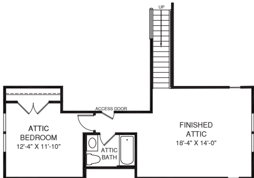
OPT. ATTIC W/ ELEVATION L & M
