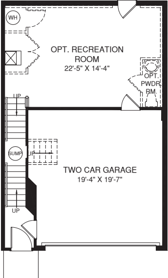
OPT. 4' EXTENSION
