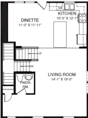
MAIN LEVEL
