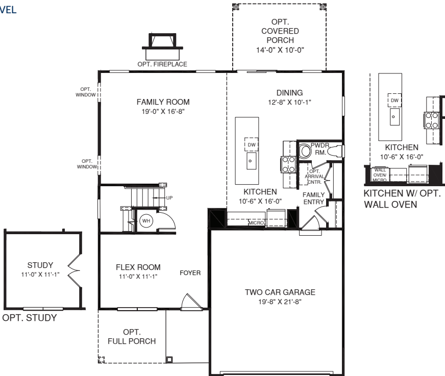
MAIN LEVEL
