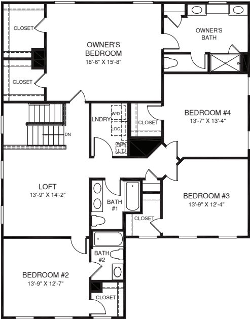
UPPER LEVEL
