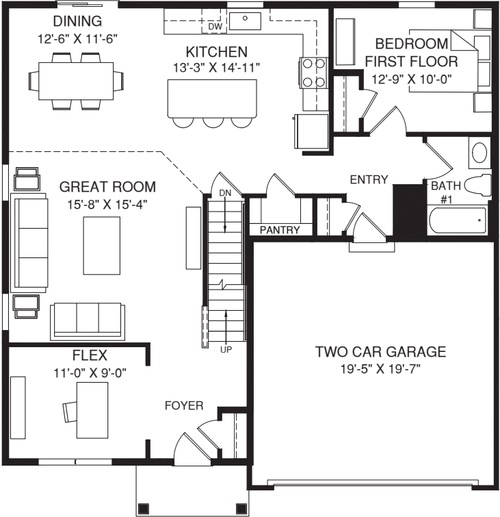
MAIN LEVEL
