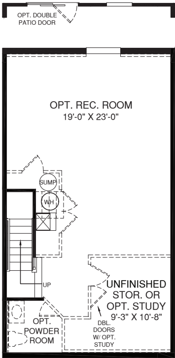
LOWER LEVEL
