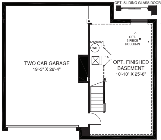
OPT. FINISHED BASEMENT SHOWN W/ MORNING ROOM
